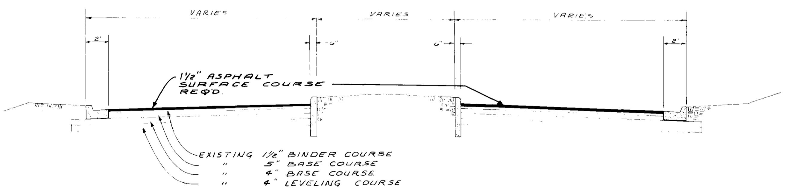
TYPICAL MEDIAN SECTION N.T.S.
