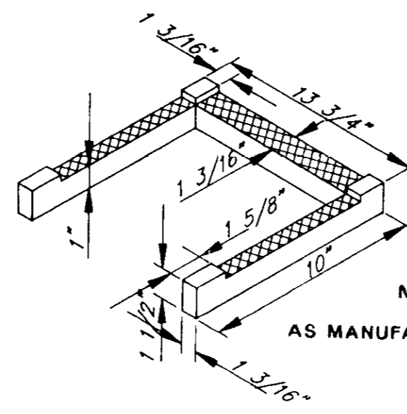
DETAIL 'B'
