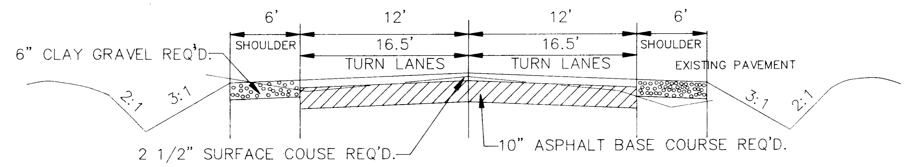
TYPICAL ROADWAY SECTION
