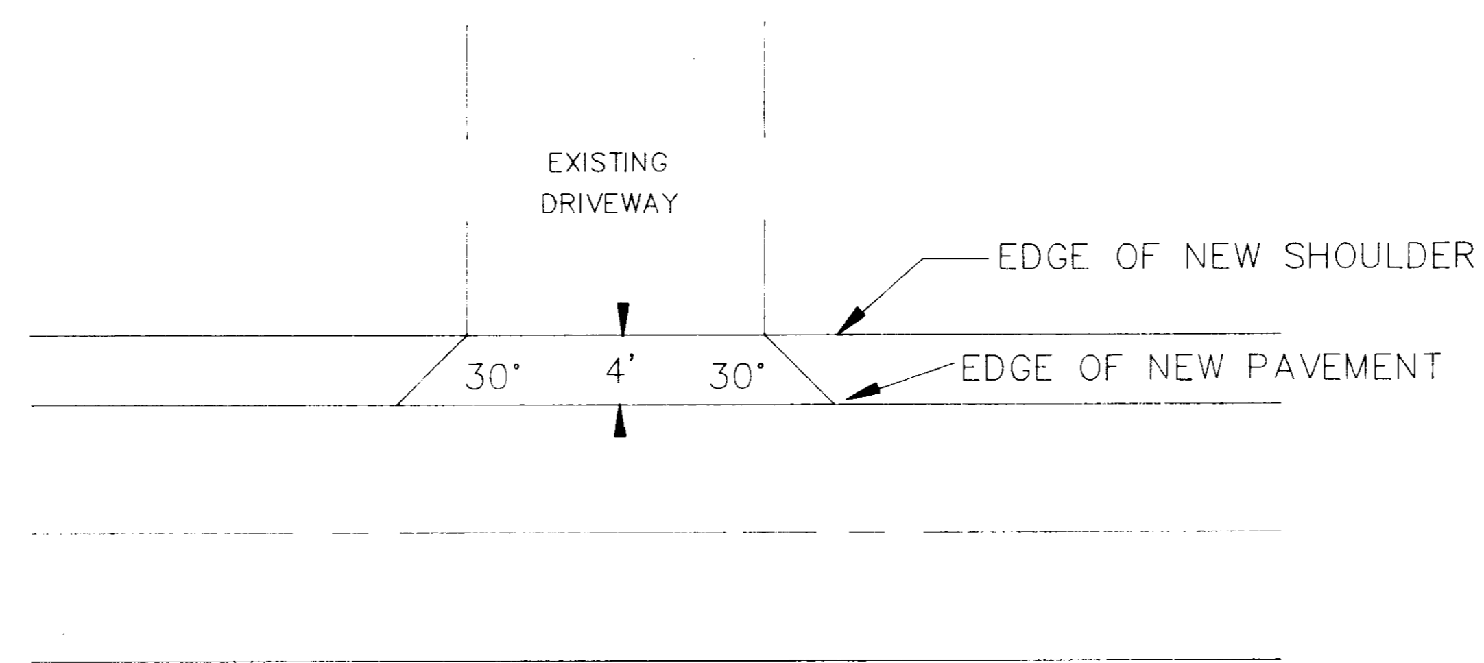
TYPICAL SECTION DRIVEWAY RAMP
